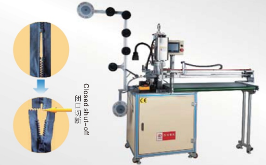
超声波切断机带机械手 Ultrasonic cutter with manipulator
