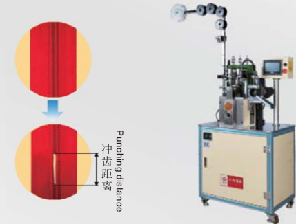
精简全自动尼龙冲齿机(全双选) automatic nylon zipper gapping machine
