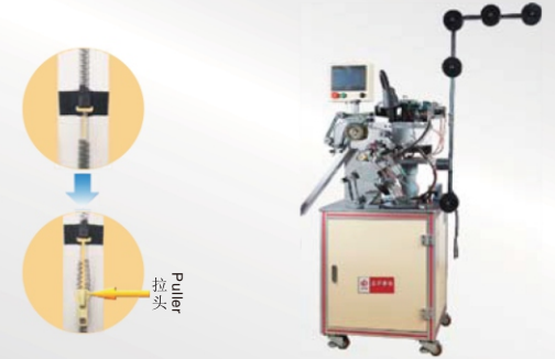
全自动穿头机(普通拉头) automatic slider wearing machine(normal slider)
