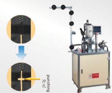
超声波冲孔机 vislon zipper ultrasonic Hole punching machine
