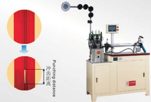
全自动尼龙冲齿机(全双选) automatic nylon zipper gapping machine
