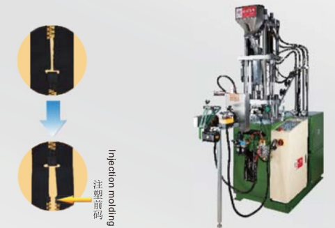
全自动闭口注塑机 fully automatic closed end bottom stopper machine
