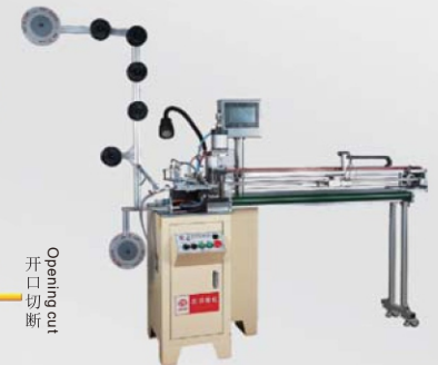
普通切断机带机械手 Ordinary cutting machine with manipulator
