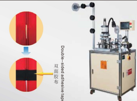
全自动尼龙双面贴布机 automatic nylon zipper sealing machine
