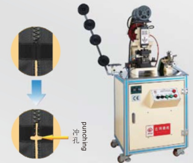
超声波冲孔机 vislon zipper ultrasonic Hole punching machine
